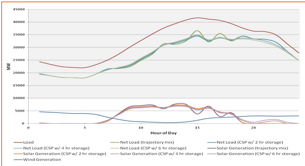
Figure 9-6: Example 2(b) - Impact of Thermal Energy Storage on High Midday Variability - additional detail on net load ramps
