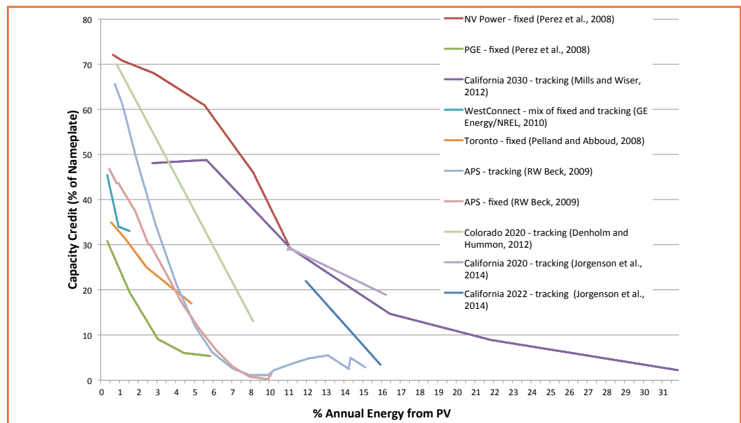
Figure 8-1: Capacity credits (% of nameplate MW) of marginal PV additions to existing portfolios from selected studies of increasing solar penetration
