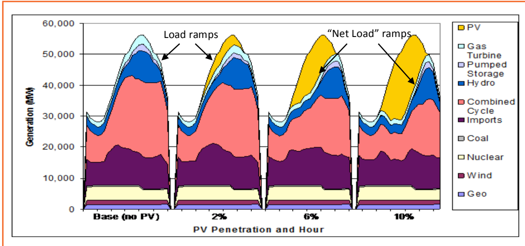
Figure 6-2: Simulated Dispatch in California for a Summer Day with PV Penetration from 0-10% Annual Energy – Comparison of Load and “Net Load” Solar Ramps
