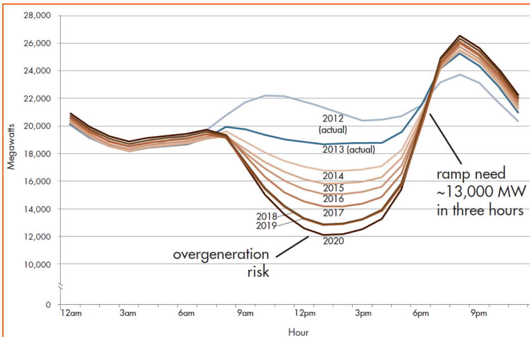
Figure 6-3: Evolution of Hourly Net Load (Wind + Solar) Ramps in the California ISO for a Spring Day, 2012-2020
