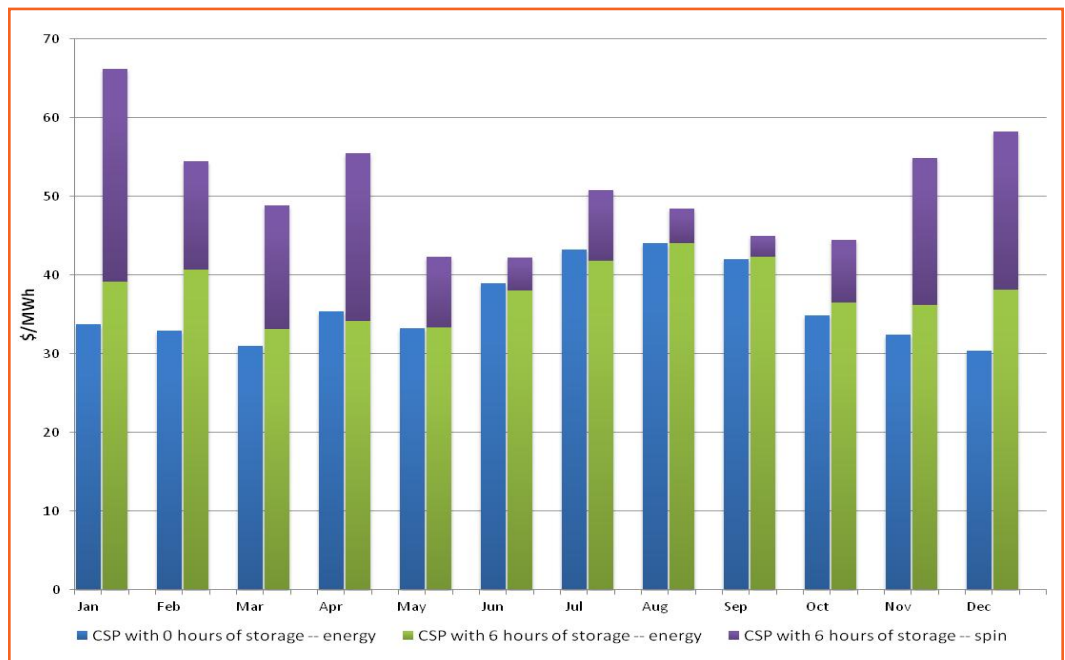
Figure 7-4: Monthly energy and spinning reserve revenues, optimized against CAISO 2011 prices
