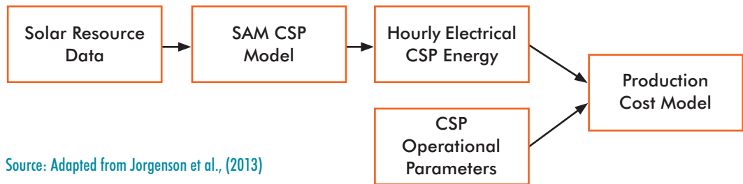
Figure 4-1: Process of simulating CSP in a production cost model developed by NREL
