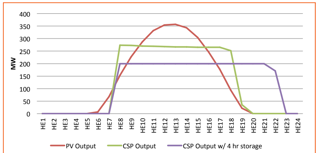
Figure 4-3: Equivalent energy production profiles on a clear day for a 200 MW CSP plant with 4 hours of storage, an approx. 275 MW CSP plant without storage, and an approx. 360 MW fixed-tilt PV plant
