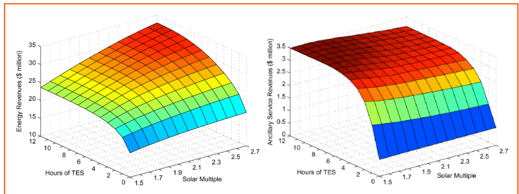
Figure 11-1: Annual revenues from energy and spinning reserves for different configurations of a parabolic trough plant, CAISO 2005 prices
