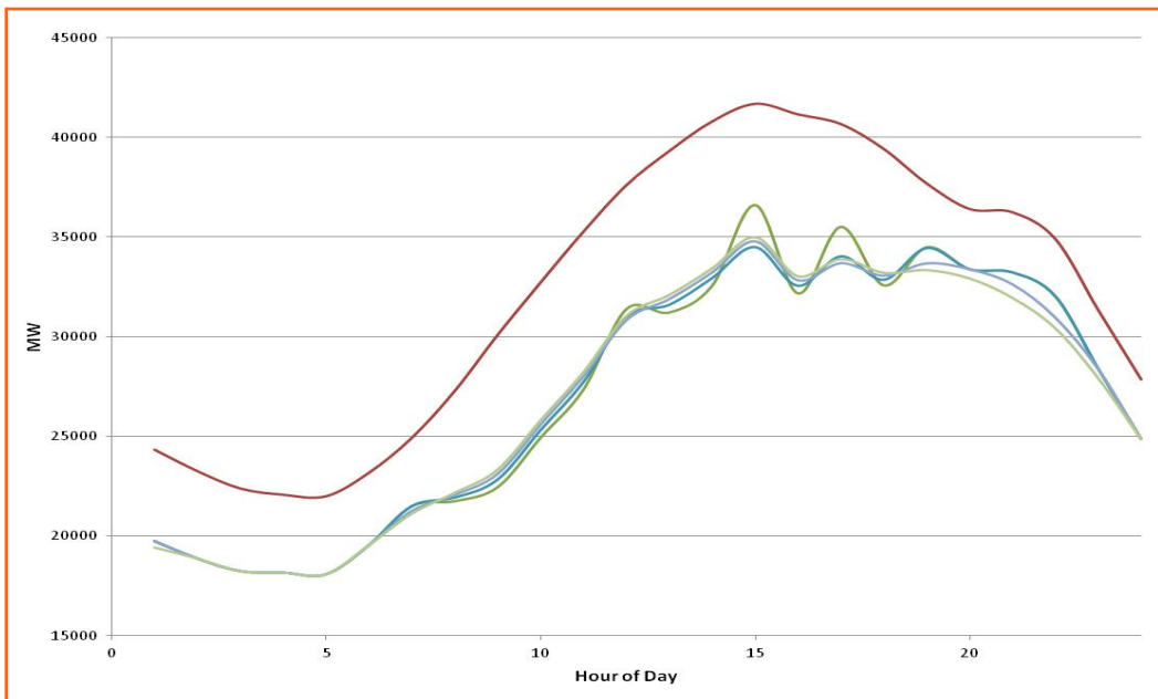
Figure 9-6: Example 2(b) - Impact of Thermal Energy Storage on High Midday Variability - additional detail on net load ramps
