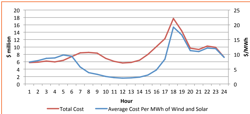
Figure 9-1: Estimated hourly distribution of integration costs in $ million and $/MWh, caused by wind and solar resources in California under 33% RPS
