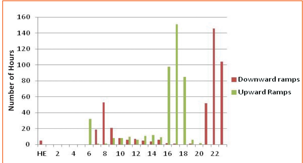
Figure 9-2: Top 10% of upward and downward net load ramp hours, by hour of day, from California ISO 2020 33% RPS Trajectory Case simulation
