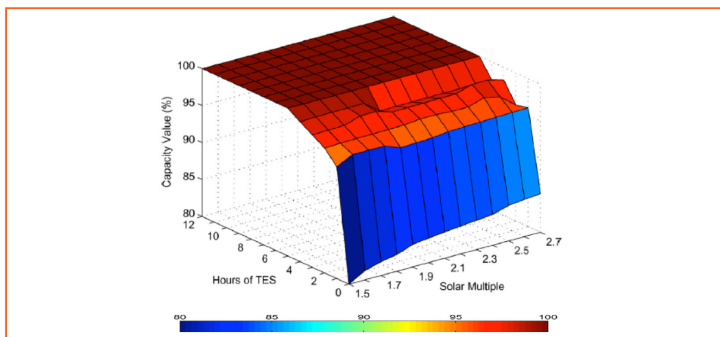
Figure 8-2: Calculation of capacity value as a percentage of nameplate capacity of a parabolic trough with and without thermal storage in Southern California (Daggett)
