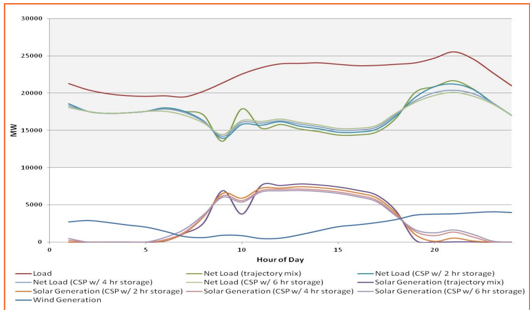
Figure 9-7: Example 3(a) - Impact of Thermal Energy Storage on rapid changes in net load – ramp direction
