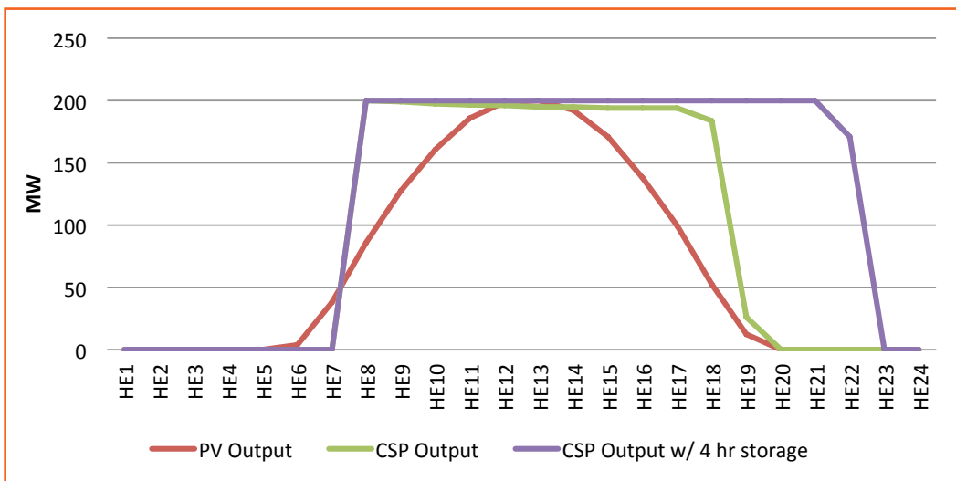
Figure 4-2: Energy production profiles for three 200 MW solar plants: fixed tilt PV plant, CSP plant without storage, and CSP plant with 4 hours of storage
