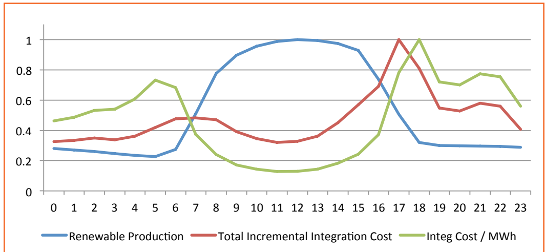
Figure B-2: Normalized Average Hourly Renewable Production (MWh), Hourly Average Integration Costs ($) and Hourly Average Integration Costs Divided by Renewable – Production ($/MWh)
