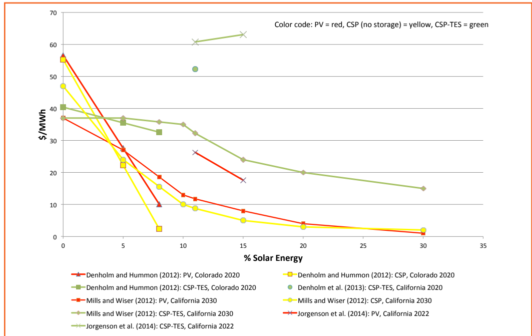
Figure 8-3: Capacity benefits ($/MWh) of solar resources from selected studies of increasing solar penetration
