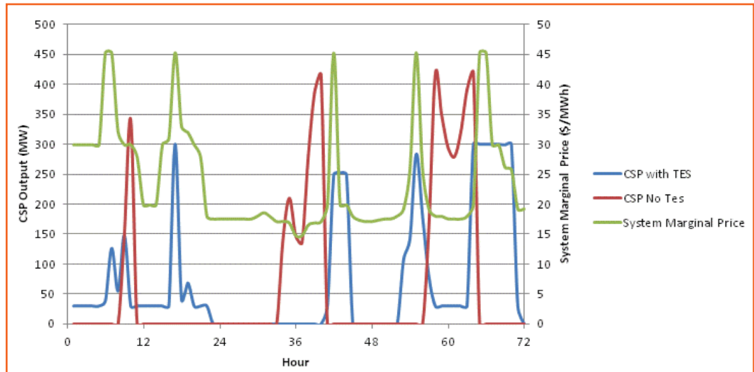
Figure 7-1: CSP with thermal energy storage dispatched against simulated January 22-24 energy prices in Colorado
