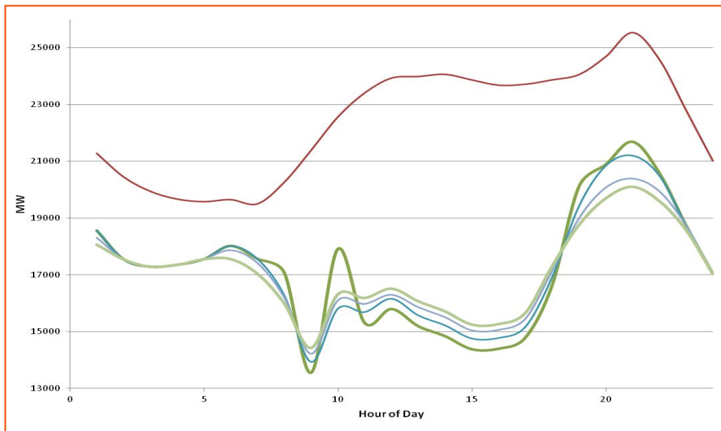
Figure 9-8: Example 3(b) - Impact of Thermal Energy Storage on rapid changes in net load ramp direction – additional detail on net load ramps
