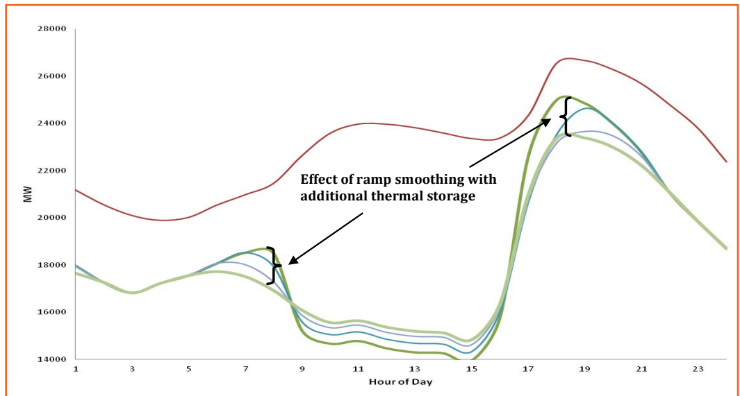
Figure 9-4: Example 1(b) - Impact of Thermal Energy Storage on High Late Afternoon – Net Load Ramp – additional detail on net load ramps
