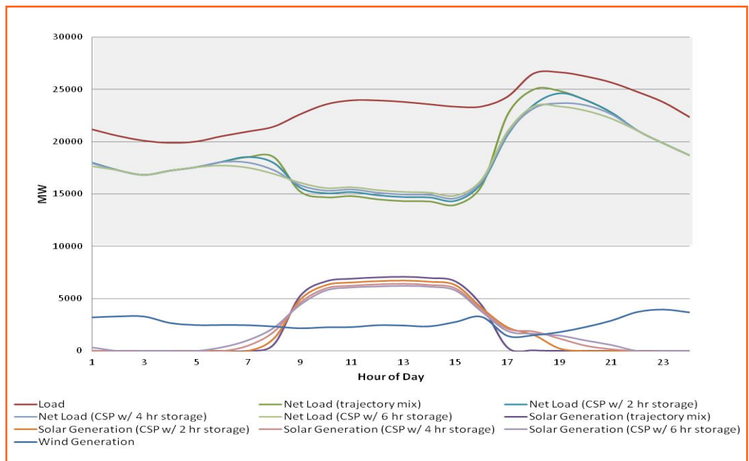
Figure 9-3: Example 1(a) - Impact of Thermal Energy Storage on High Late Afternoon – Net Load Ramp
