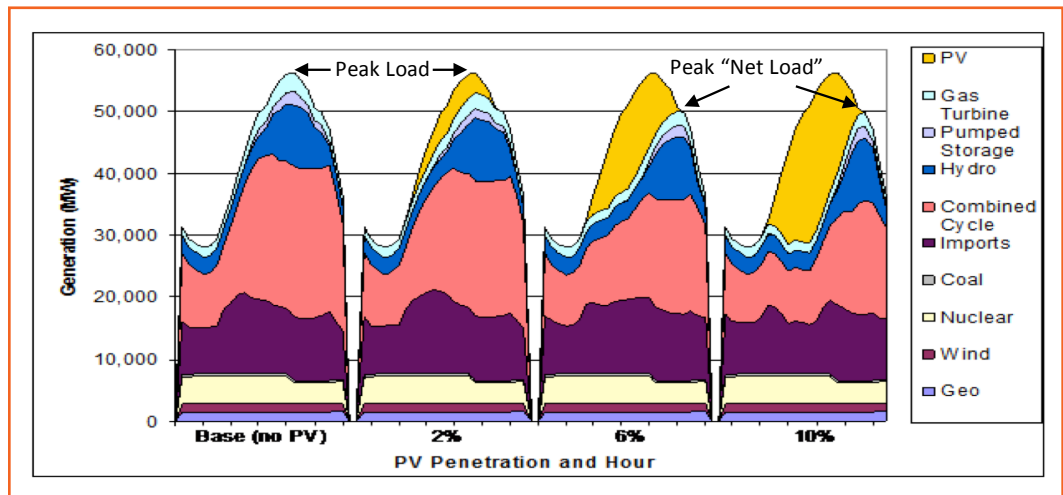
Figure 6-1: Simulated Dispatch in California for a Summer Day with PV Penetration from 0-10% Annual Energy – Comparison of Peak Load and Peak “Net Load”
